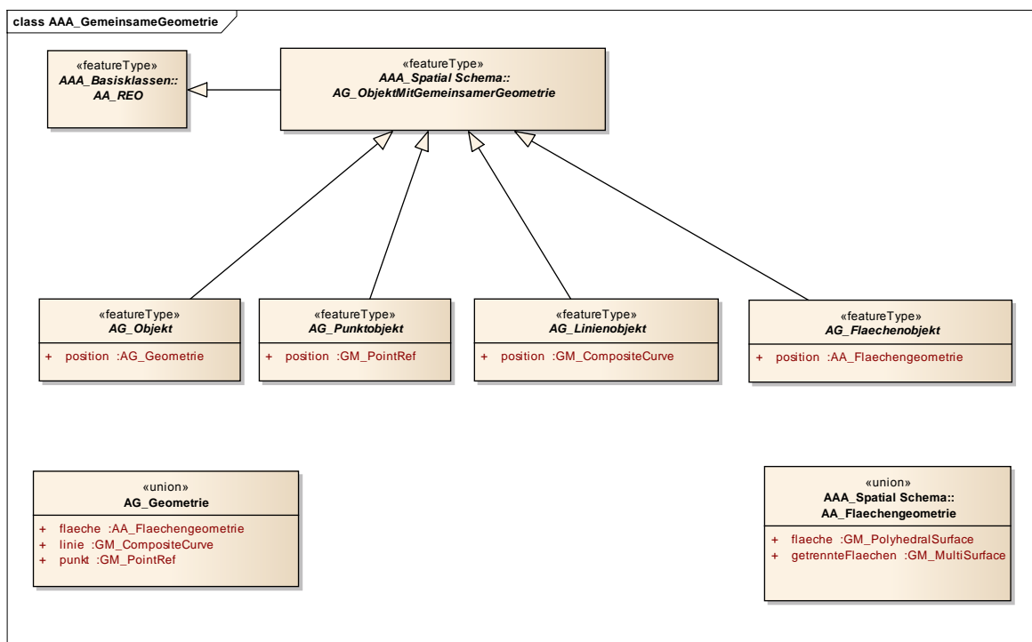
Figure 11: Objects with jointly used geometry
