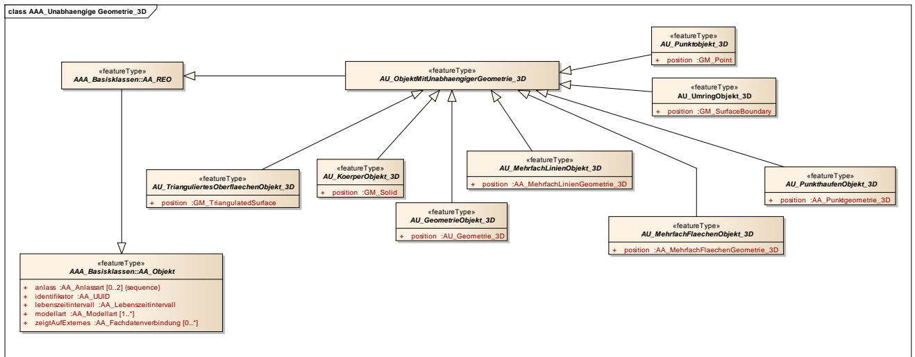
Figure 14: 3D objects with independent geometry
