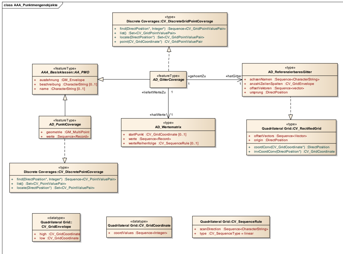
Figure 18: Modelling of the Point Coverage Classes
