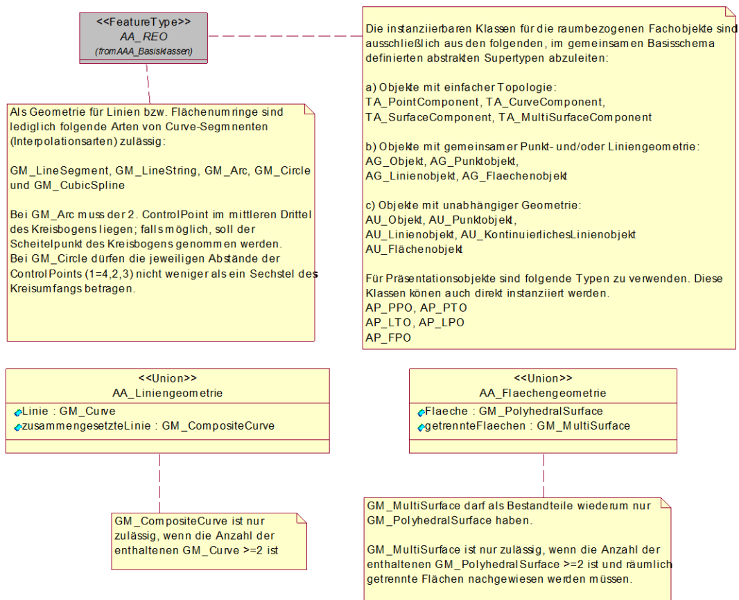
Figure 10: Geometry and instantiable classes
