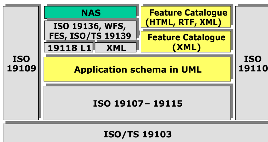
Figure 36: Embedding the NAS in de-jure standards and de-facto standards
