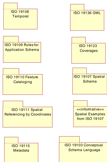
Figure 4: Components of the ISO 19100 series of standards used
