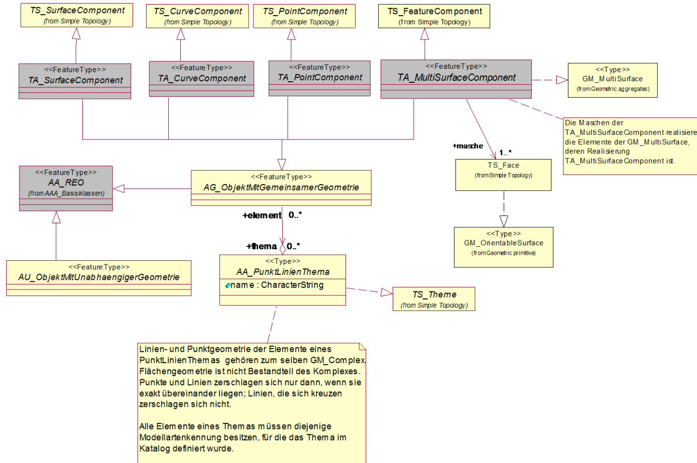
Figure 9: Summary of the enhancements to the standardised Spatial Schema required by AFIS-ALKIS-ATKIS
