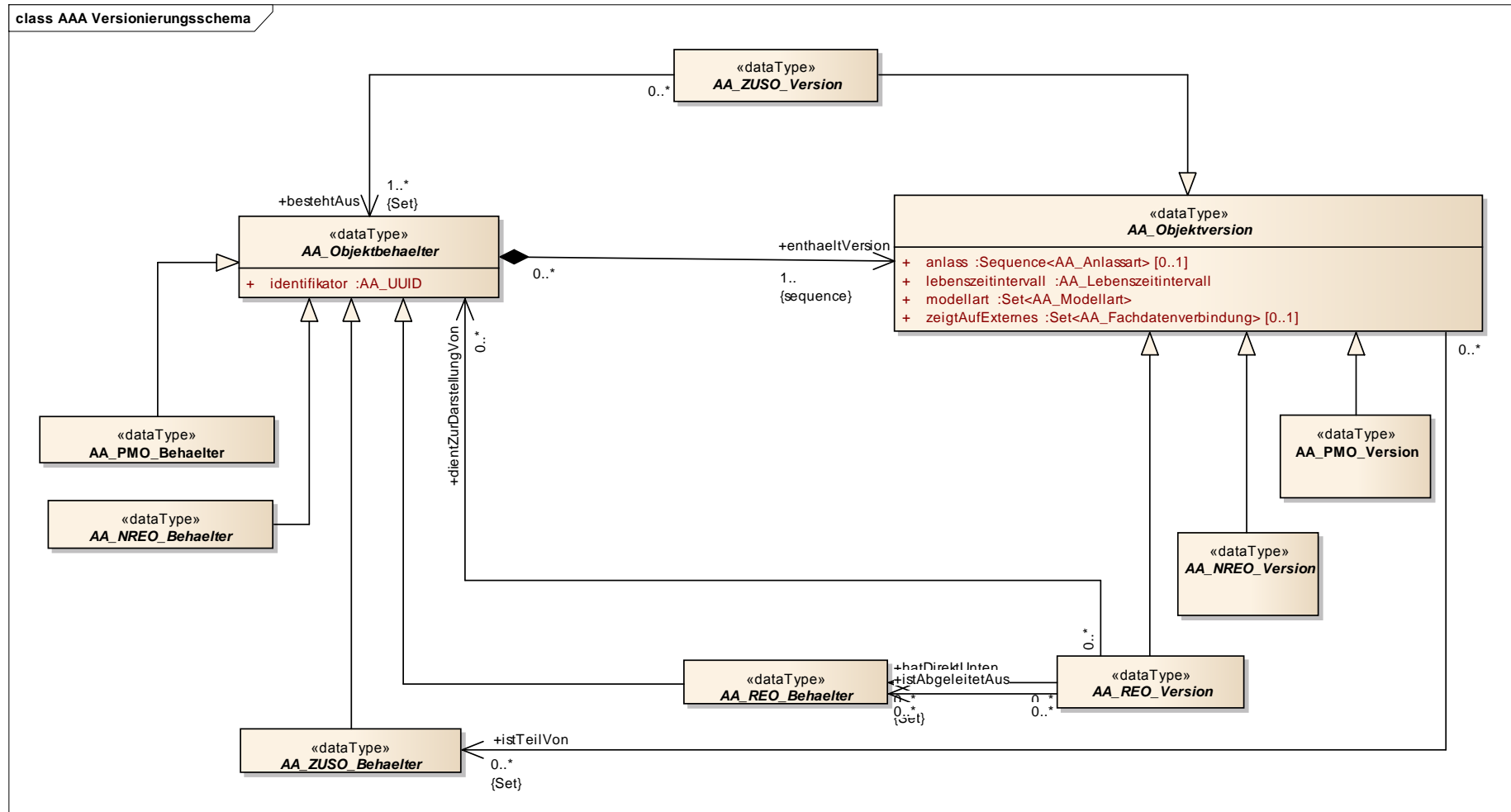
Figure 24: Versioning schema
