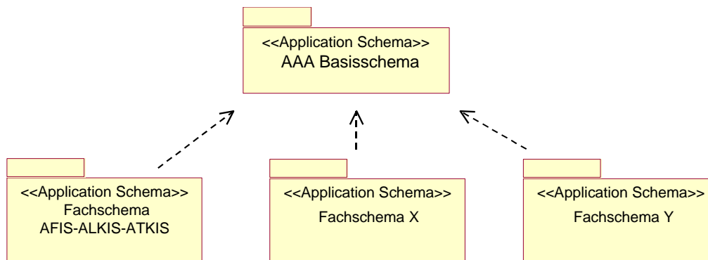
Figure 6: The basic schema as a basis for application-specific domain schemas (e.g. AFIS, ALKIS and ATKIS)
