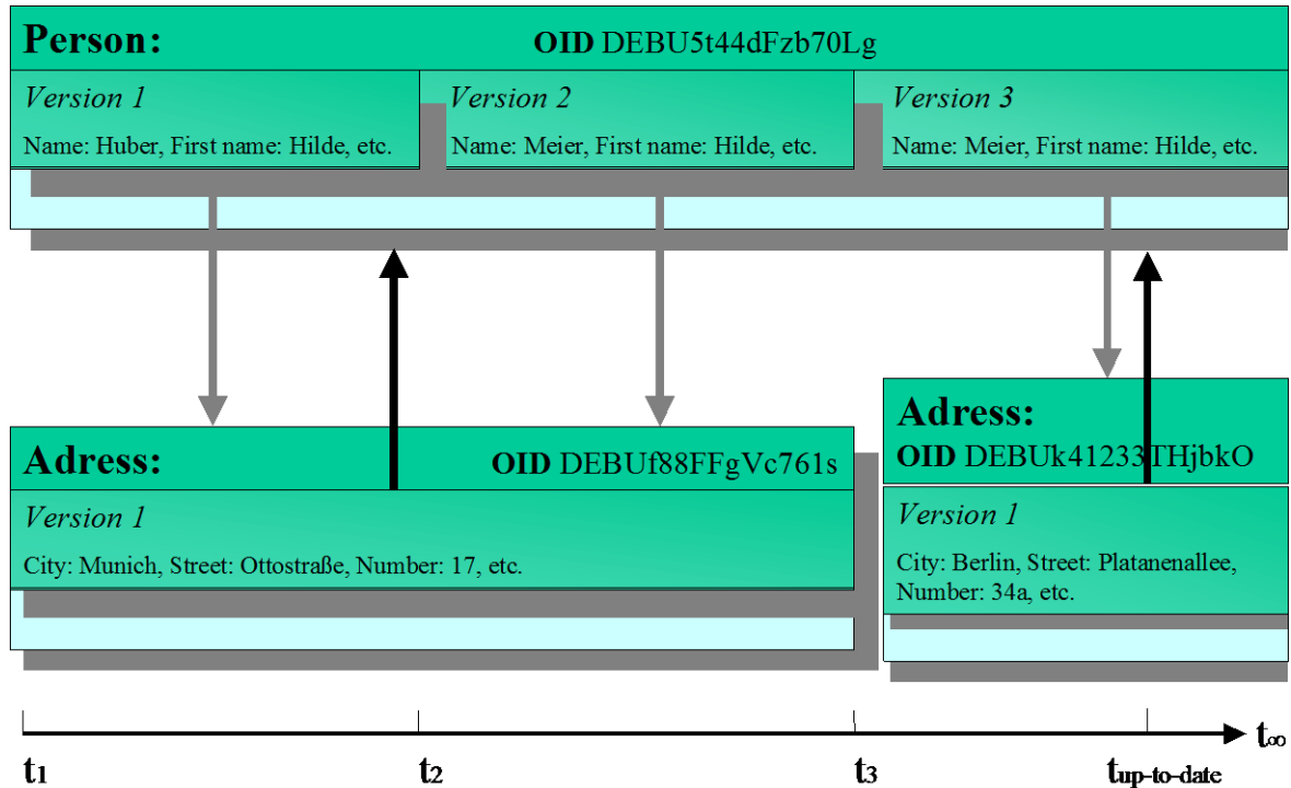
Figure 26: Example of versioning following change of relations
