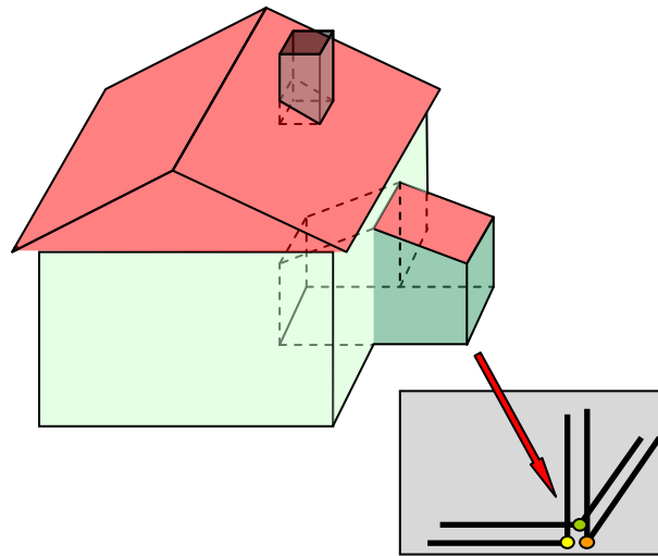
Figure 11: Features with independent 3D geometry
