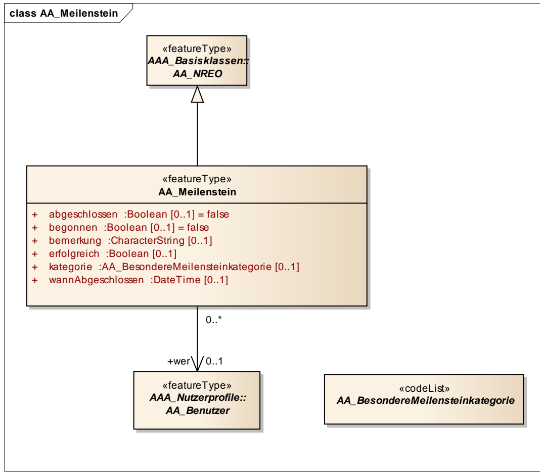
Figure 34: "AA_Milestone" (AA_Meilenstein) class diagram
