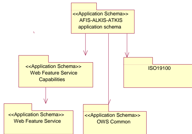
Figure 3: Dependency of the AFIS-ALKIS-ATKIS application schema on the structures standardised by ISO 19100 and OGC
