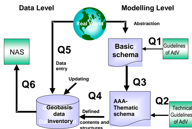
Figure 40: The quality assurance model of the AFIS-ALKIS-ATKIS project
