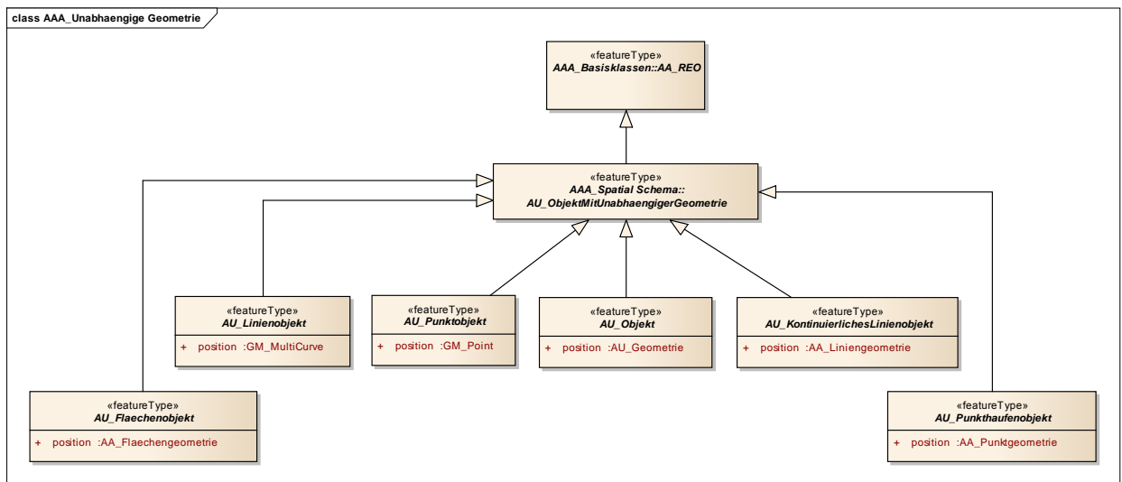
Figure 13: 2D objects with independent geometry
