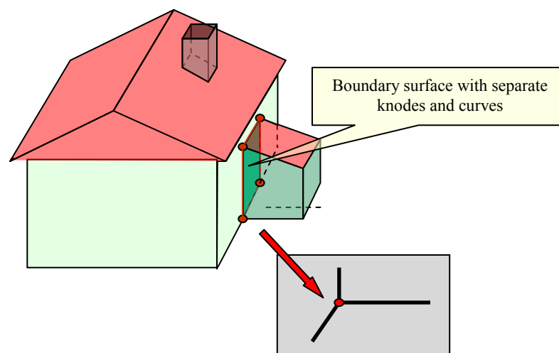
Figure 10: 3D-features with jointly used geometry
