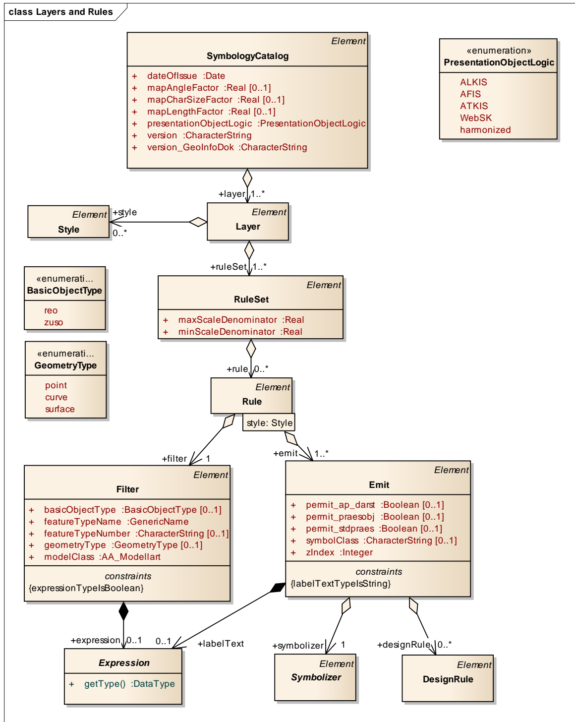
Figure 28: Schema of SK object model
