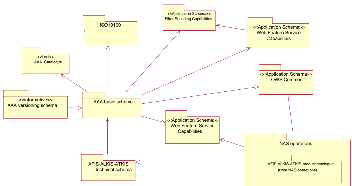
Figure 5: The components of the AFIS-ALKIS-ATKIS application schema
