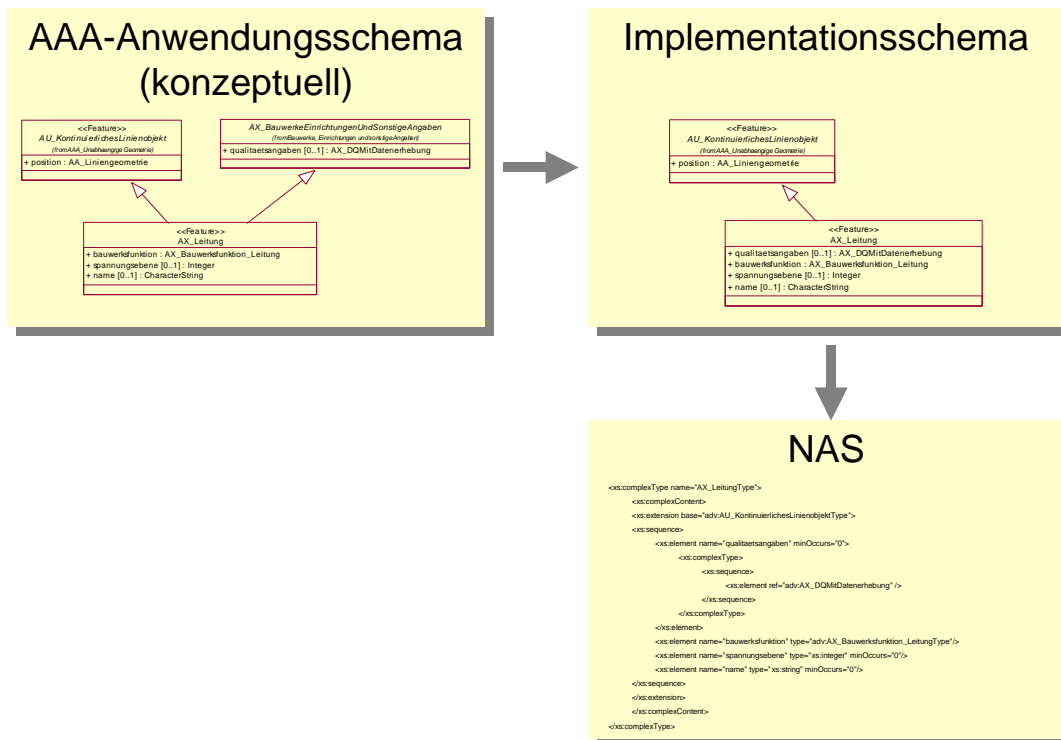
Figure 35: Two level derivation process of the NAS
