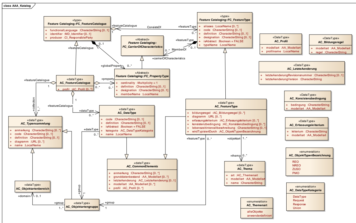
Figure 27: Expansion of standardised structure of the feature catalogues
