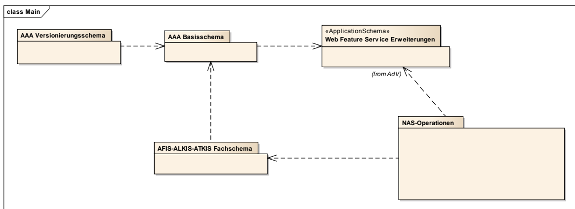
Figure 39: UML package "NAS-operations" in the context of application schema components
