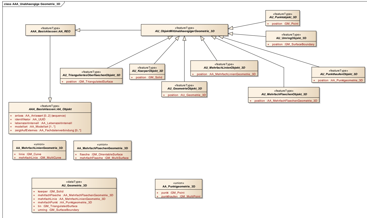
Figure 12: Features with independent 3D geometry
