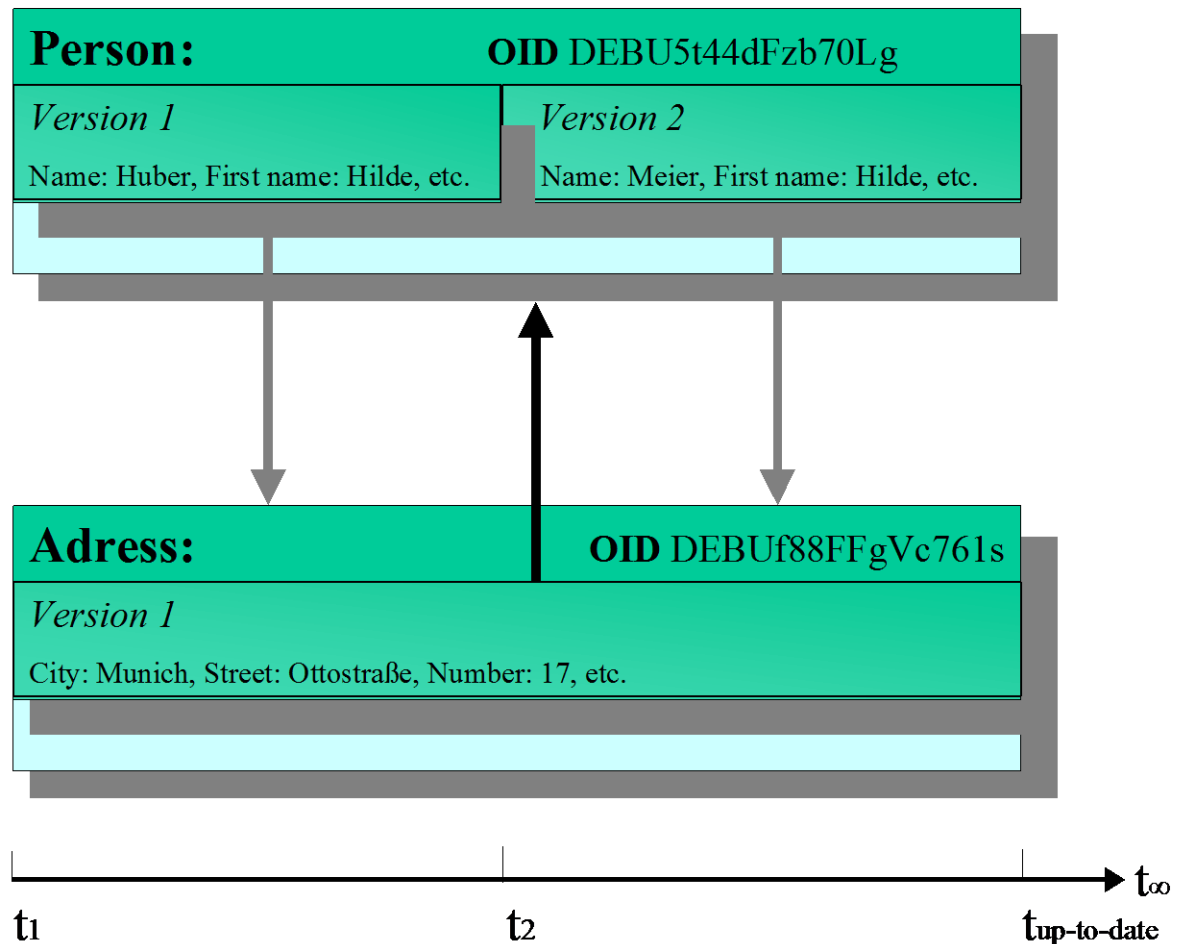
Figure 25: Example of versioning following change of attributes
