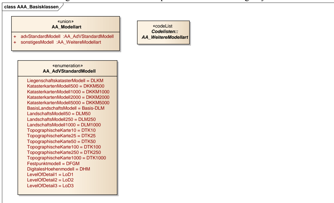
Figure 19: Model types in the Basic Schema
