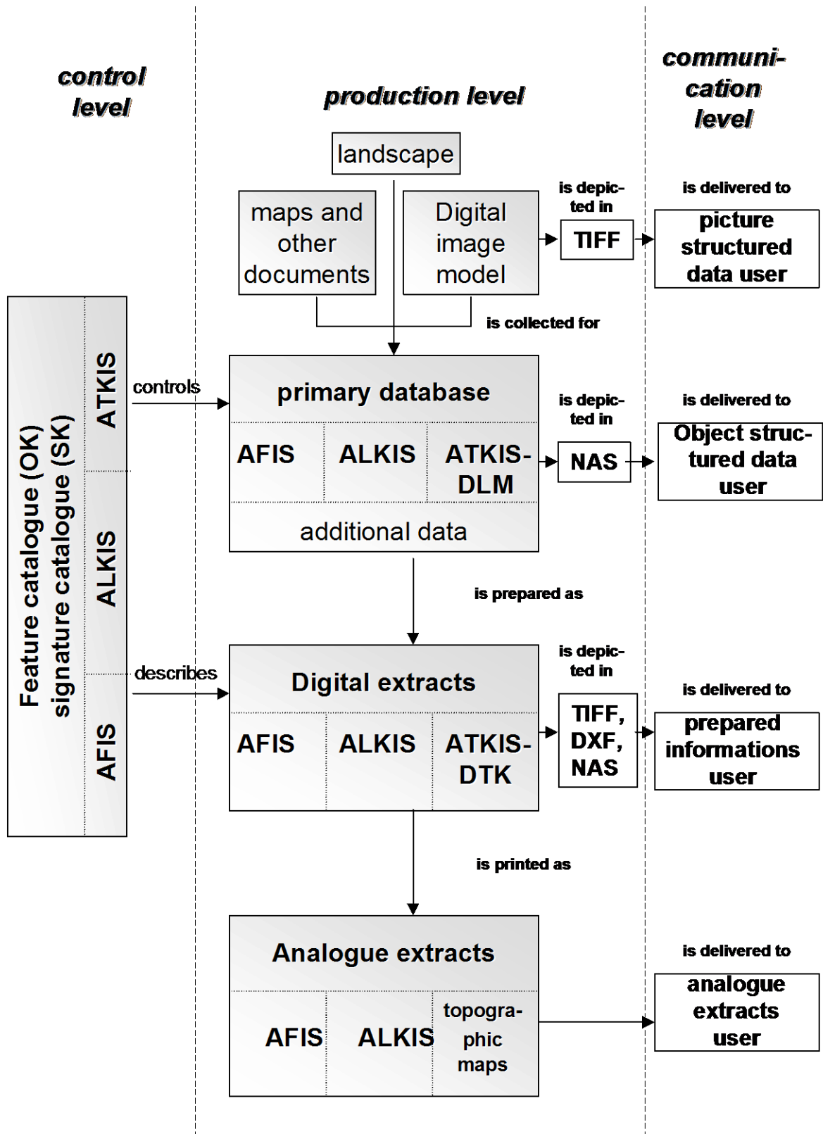
Figure 1: Common AFIS-ALKIS-ATKIS Reference Model (Source: The common AFIS-ALKIS-ATKIS Reference Model, 1996)
